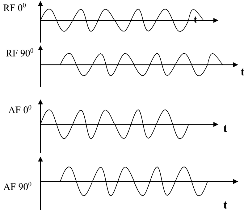
Balanced Modulator o/p - 1
